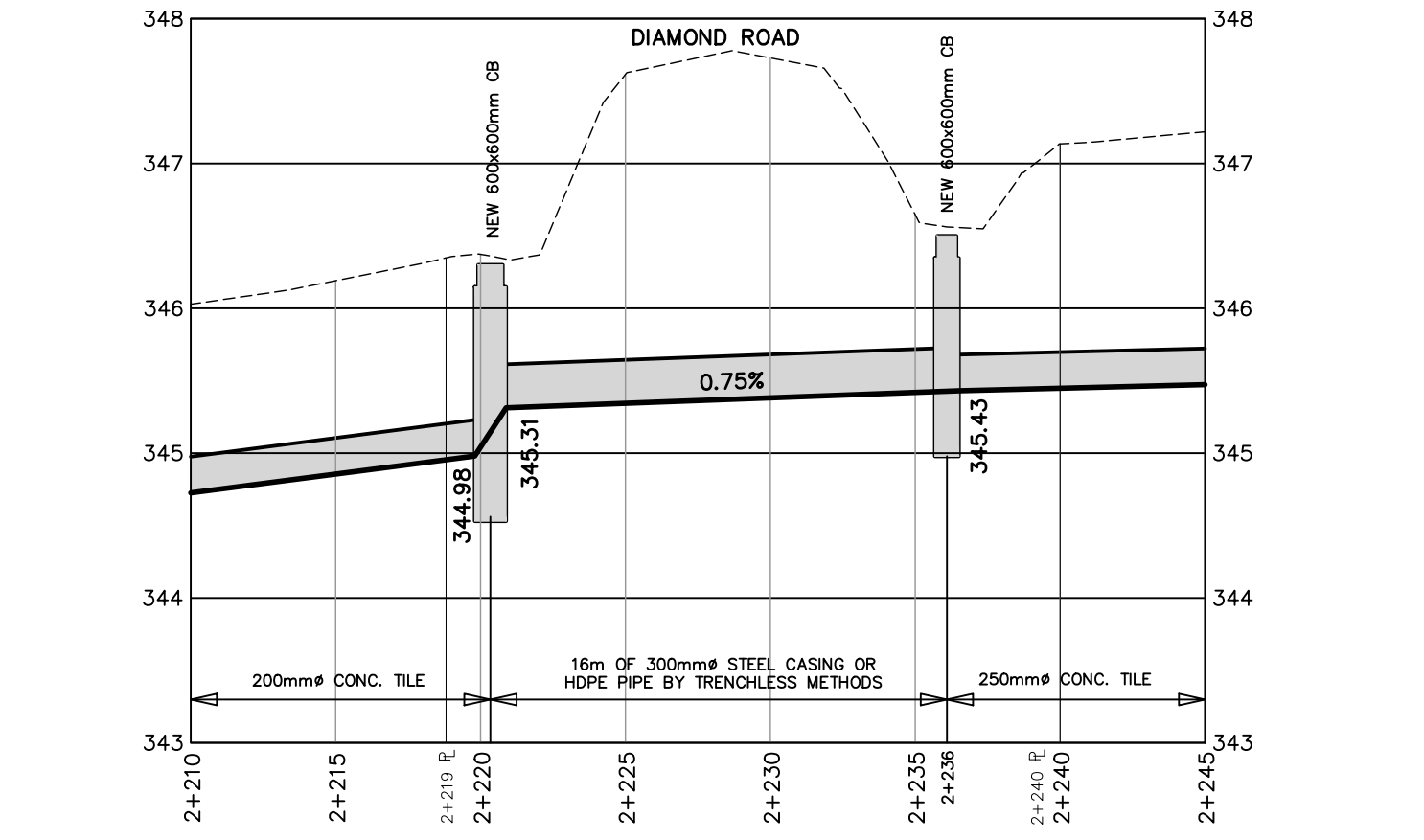
DIAMOND ROAD CROSSING – MAIN DRAIN
