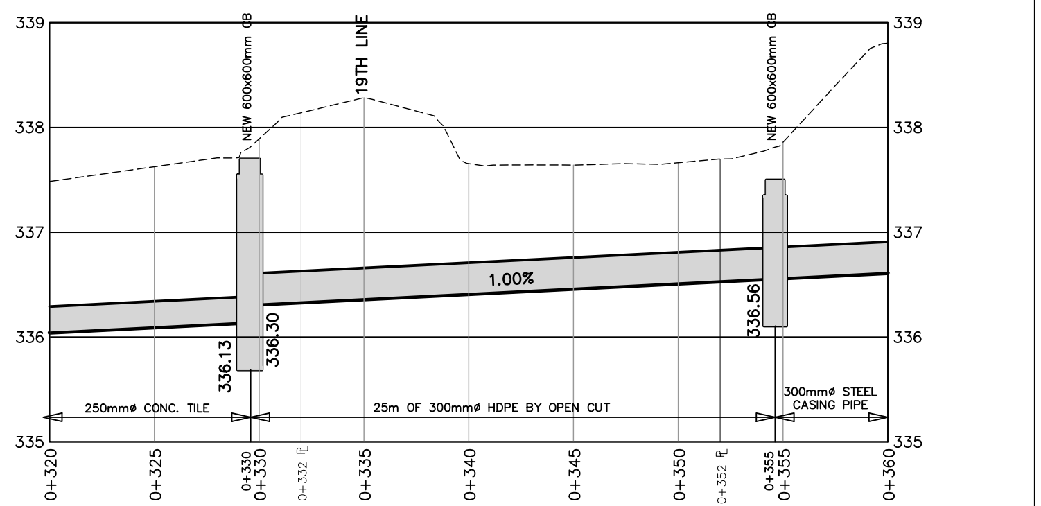
19TH LINE CROSSING - BRANCH 2
