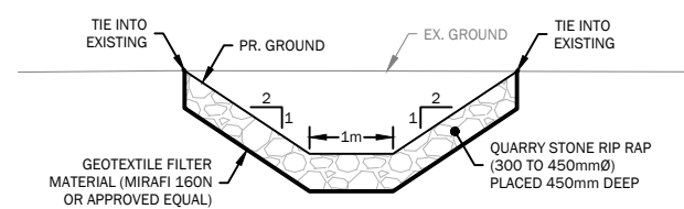
TYPICAL SWALE DETAIL N.T.S.
